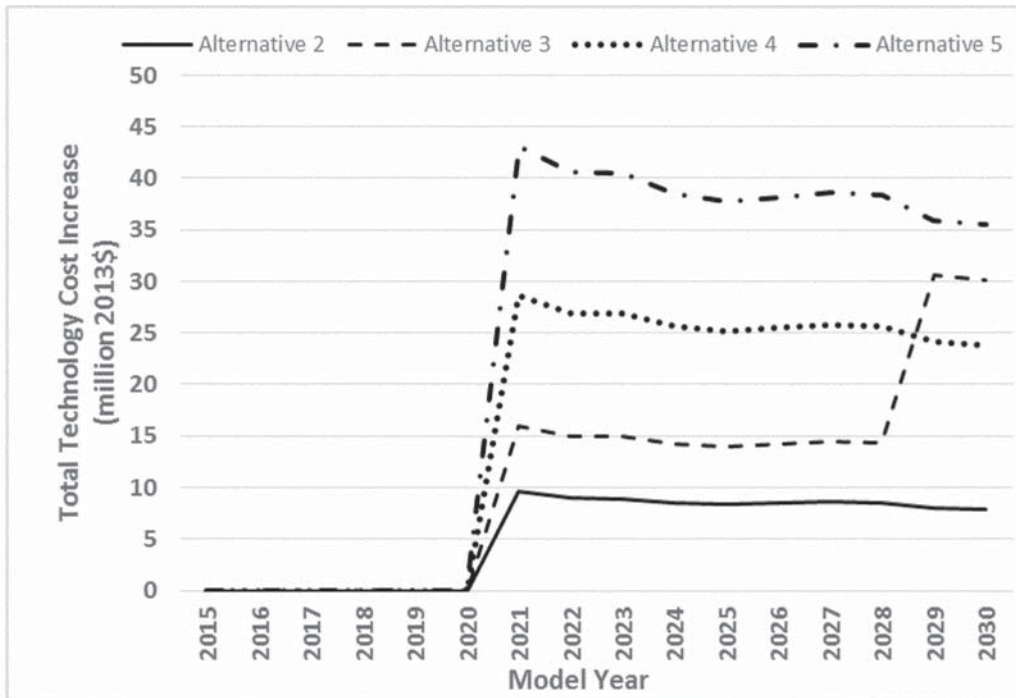
Figure VI-27 Total Technology Cost Increase for Nissan by Model Year and Alternative
